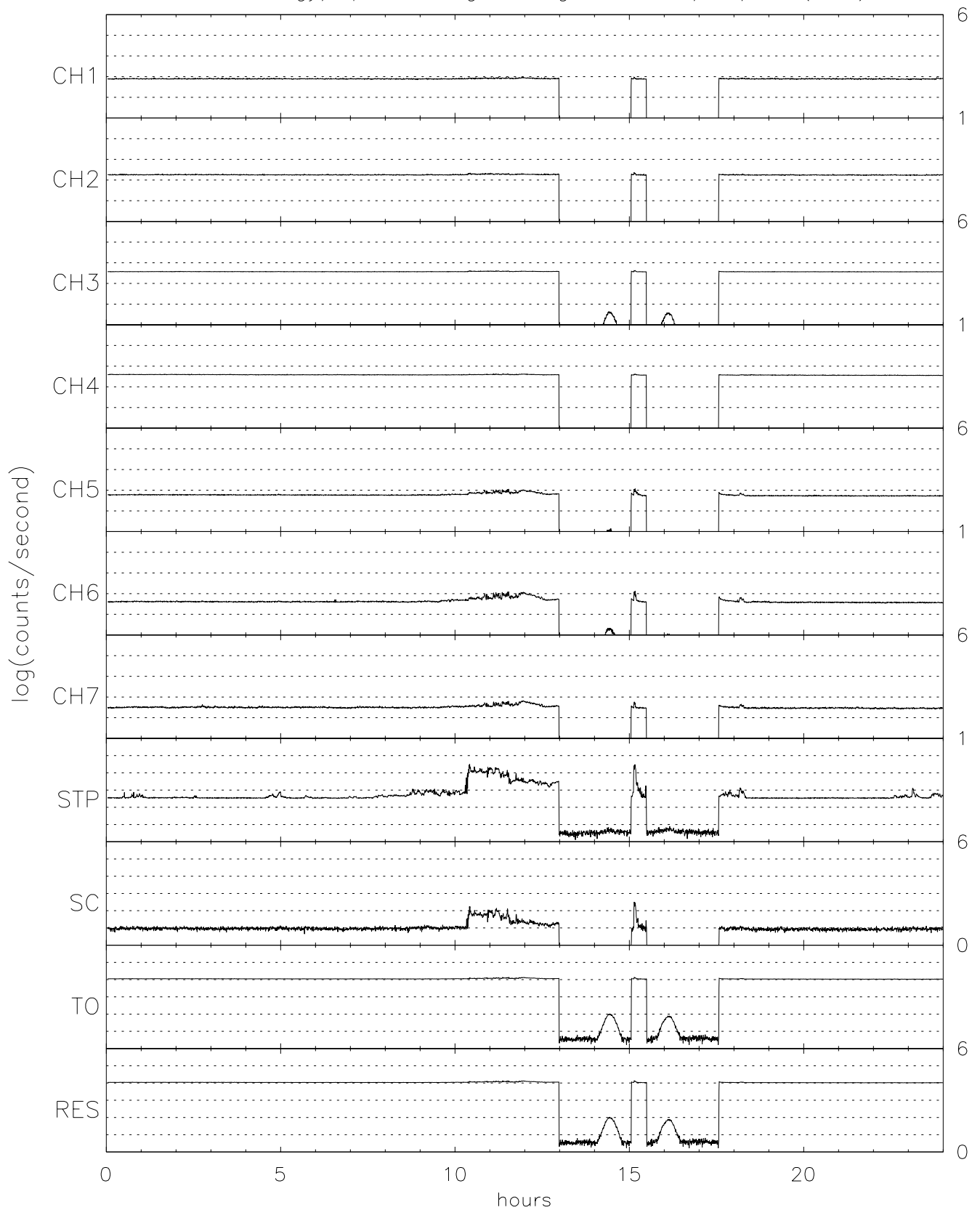
TIDE energy/spin averaged Singles for 12/04/96 (339)
