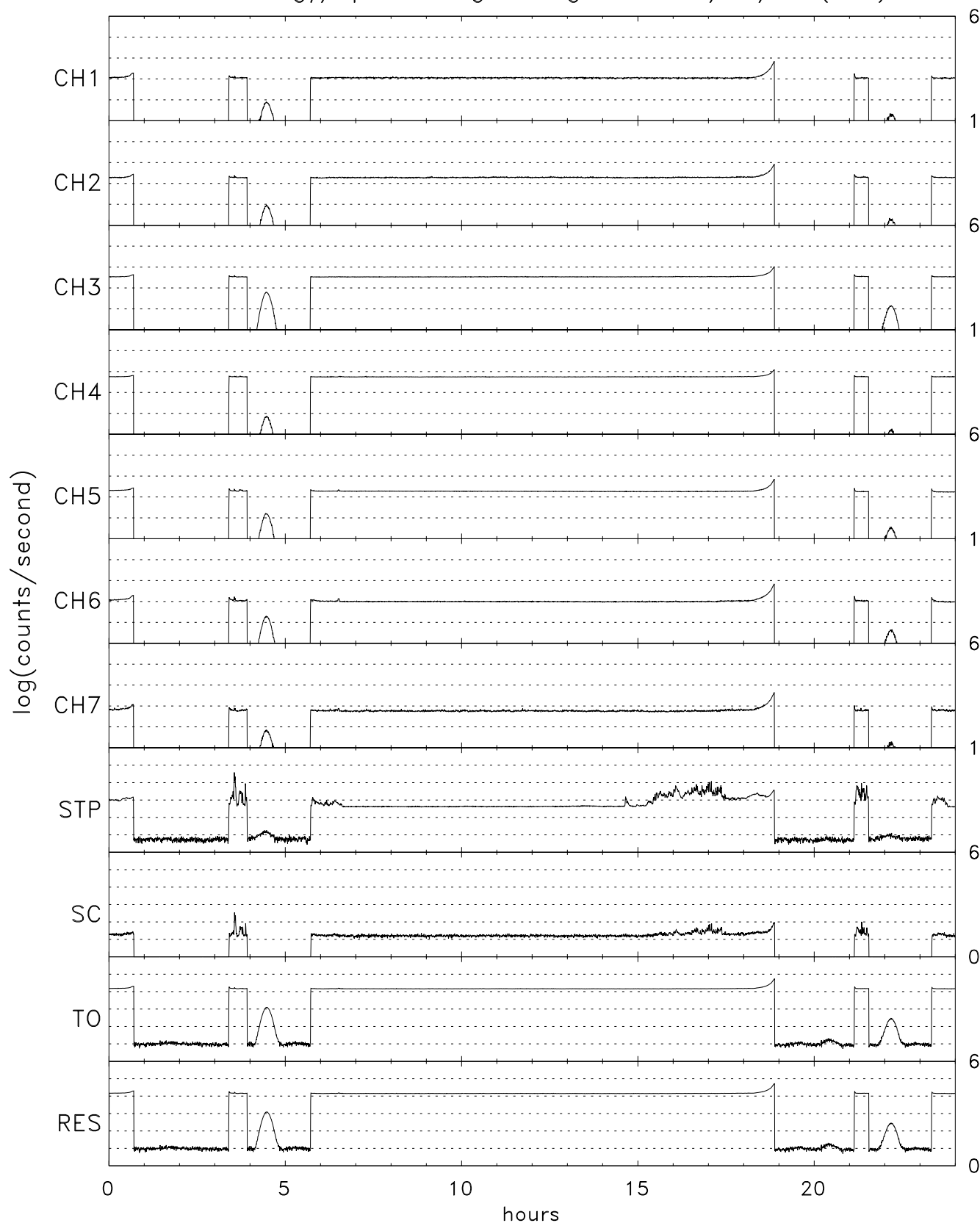
TIDE energy/spin averaged Singles for 11/22/96 (327)
