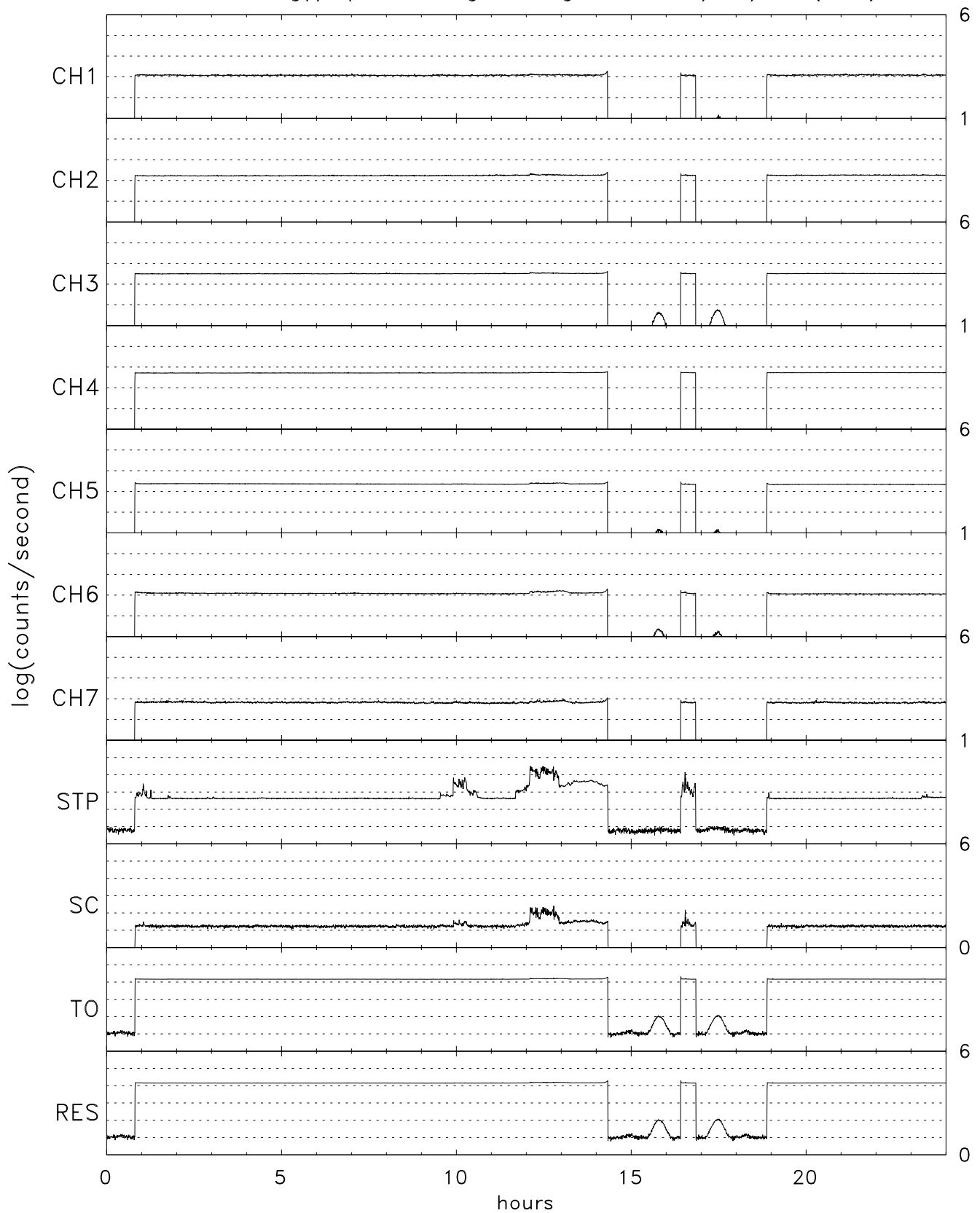
TIDE energy/spin averaged Singles for 11/20/96 (325)
