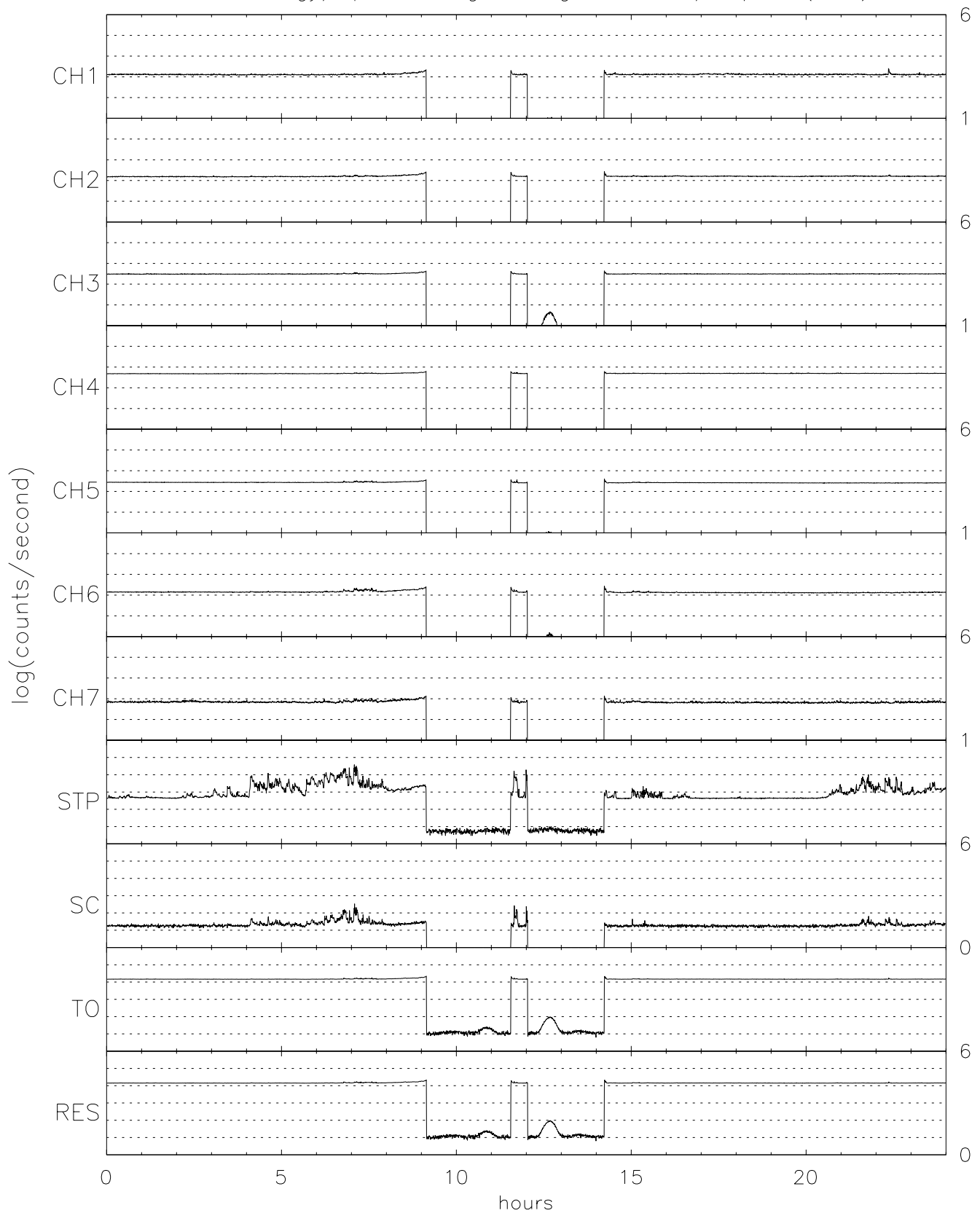
TIDE energy/spin averaged Singles for 11/18/96 (323)
