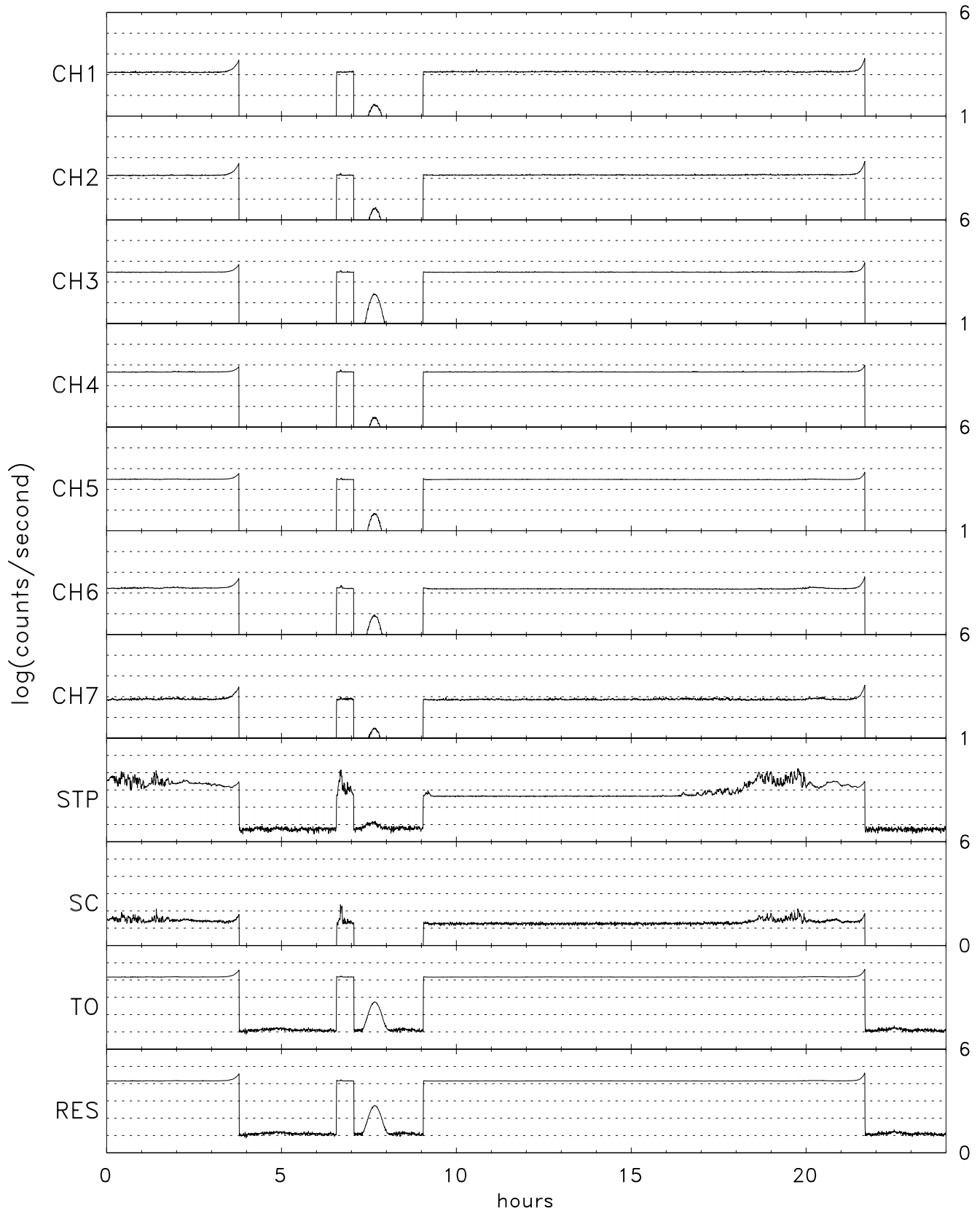
TIDE energy/spin averaged Singles for 11/16/96 (321)
