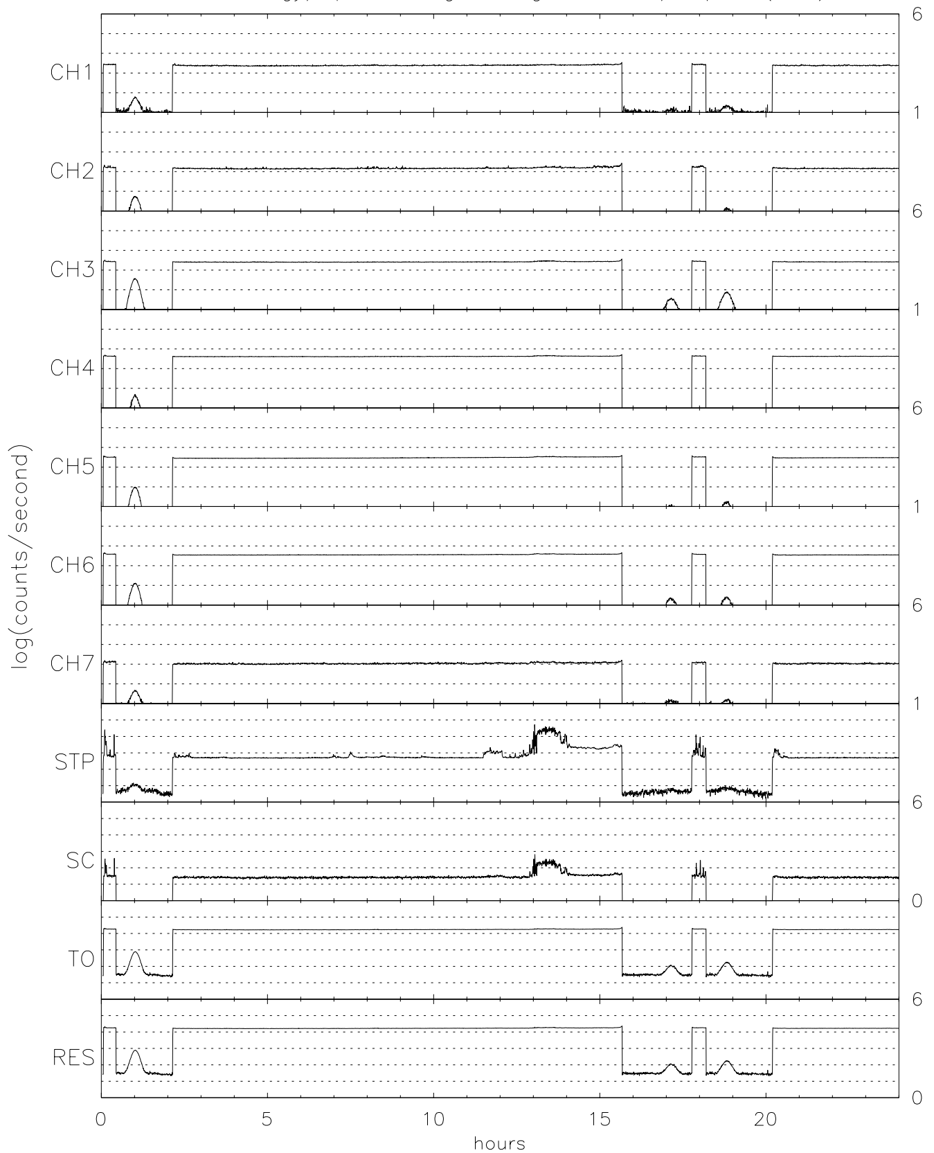
TIDE energy/spin averaged Singles for 11/06/96 (311)
