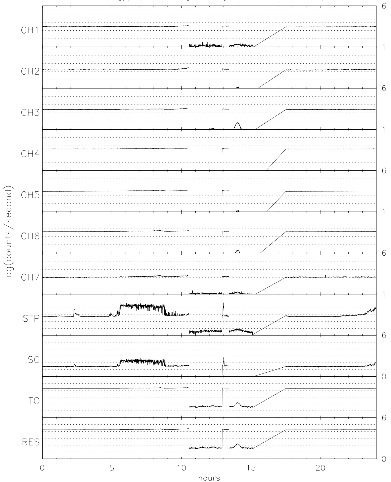
TIDE energy/spin averaged Singles for 11/04/96 (309)
