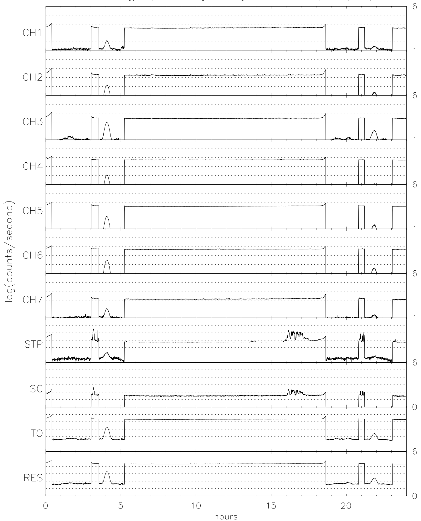
TIDE energy/spin averaged Singles for 10/31/96 (305)
