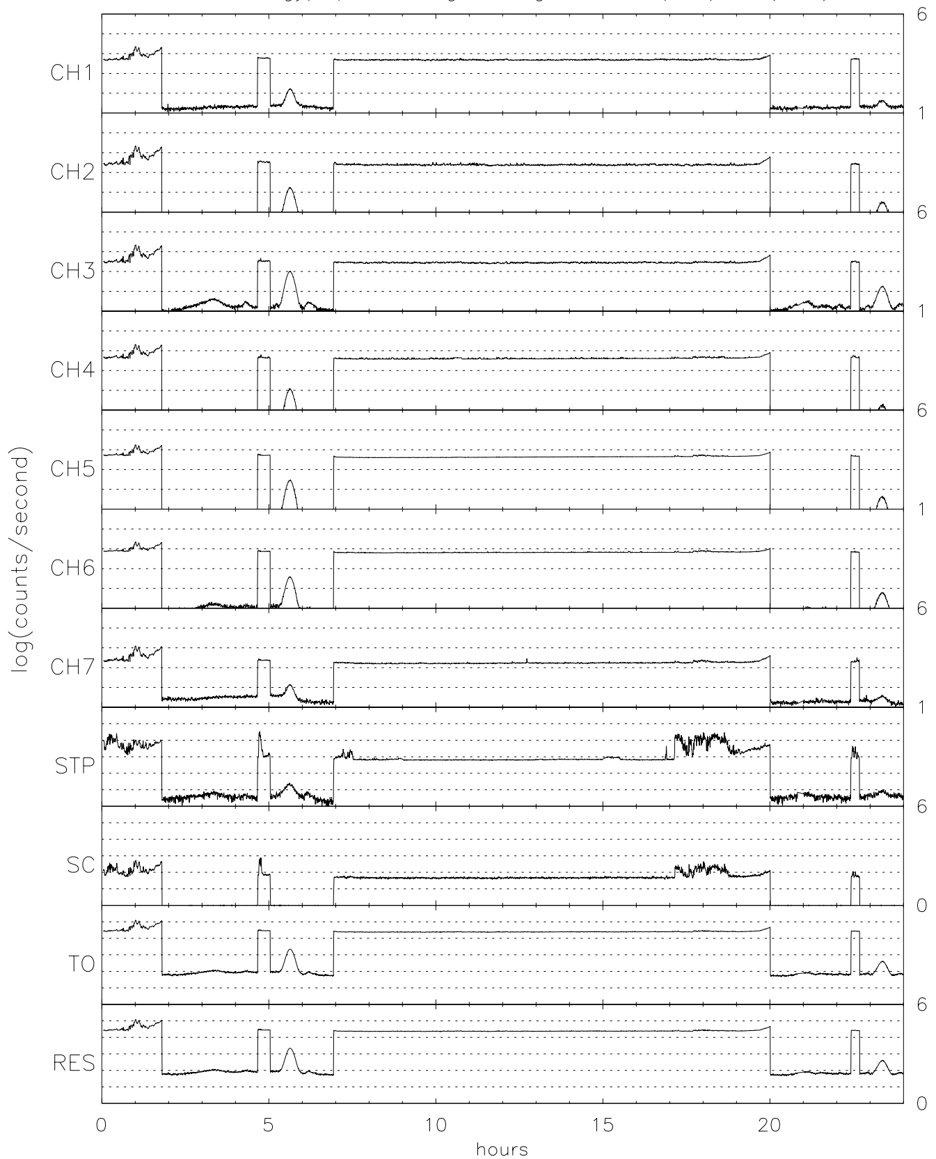
TIDE energy/spin averaged Singles for 10/28/96 (302)
