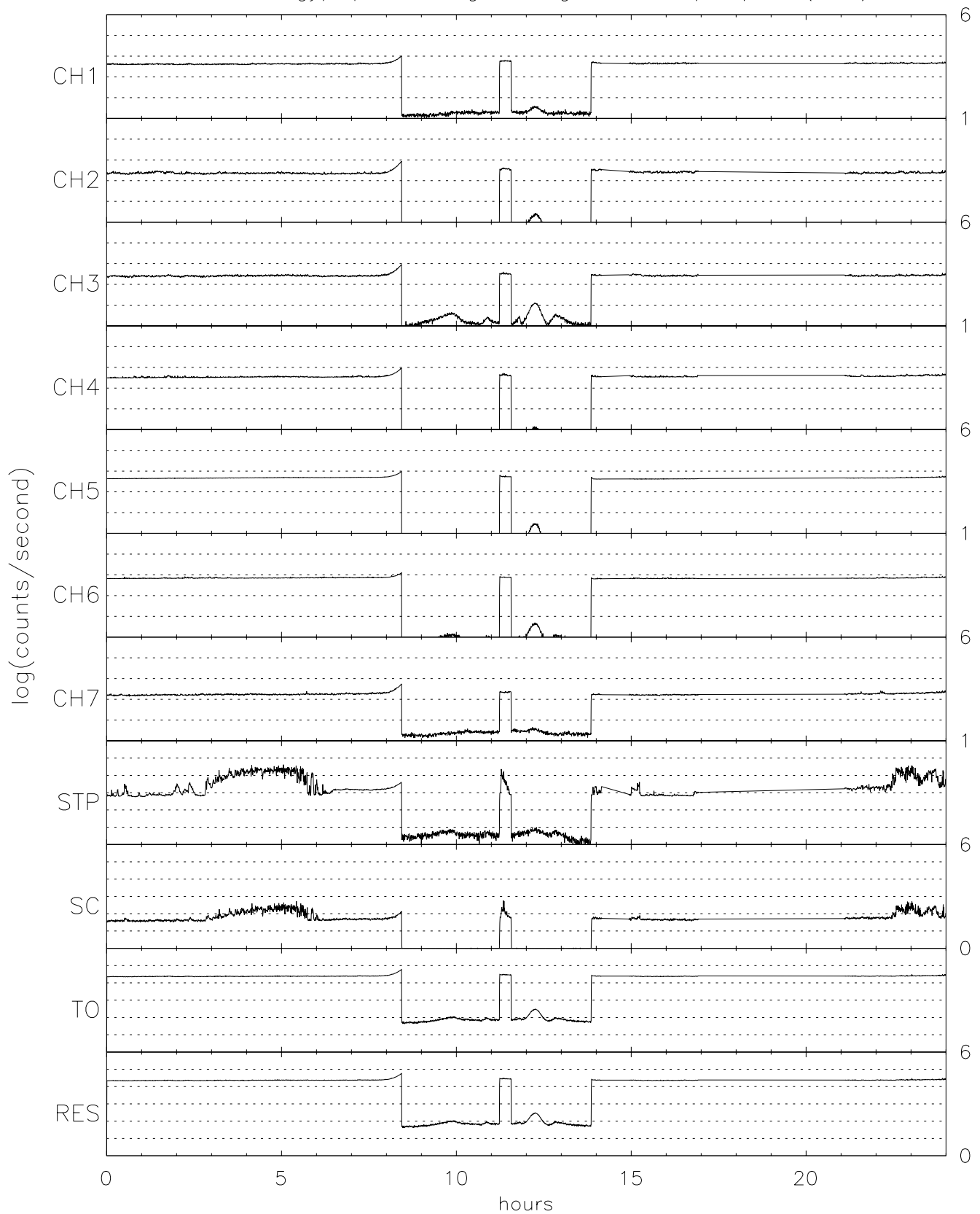
TIDE energy/spin averaged Singles for 10/27/96 (301)
