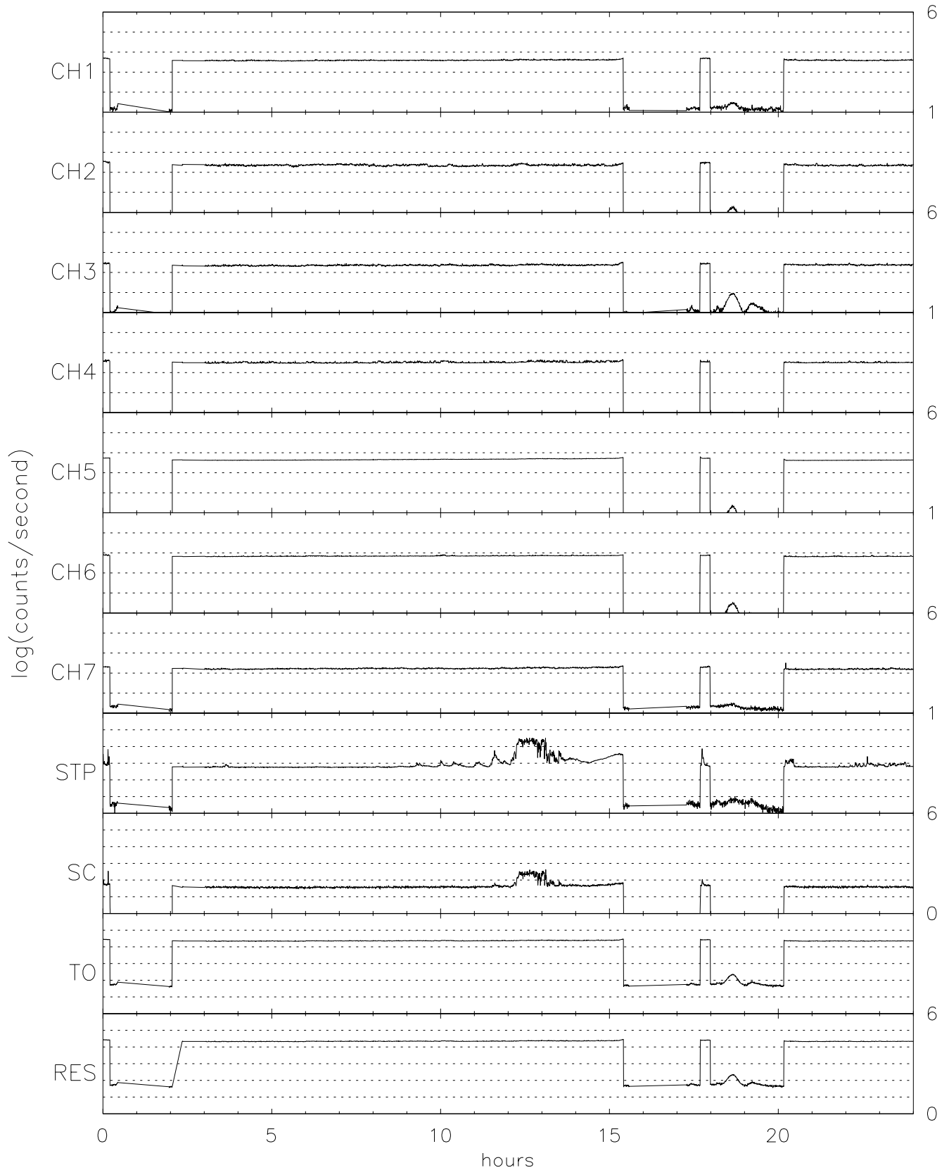
TIDE energy/spin averaged Singles for 10/26/96 (301)
