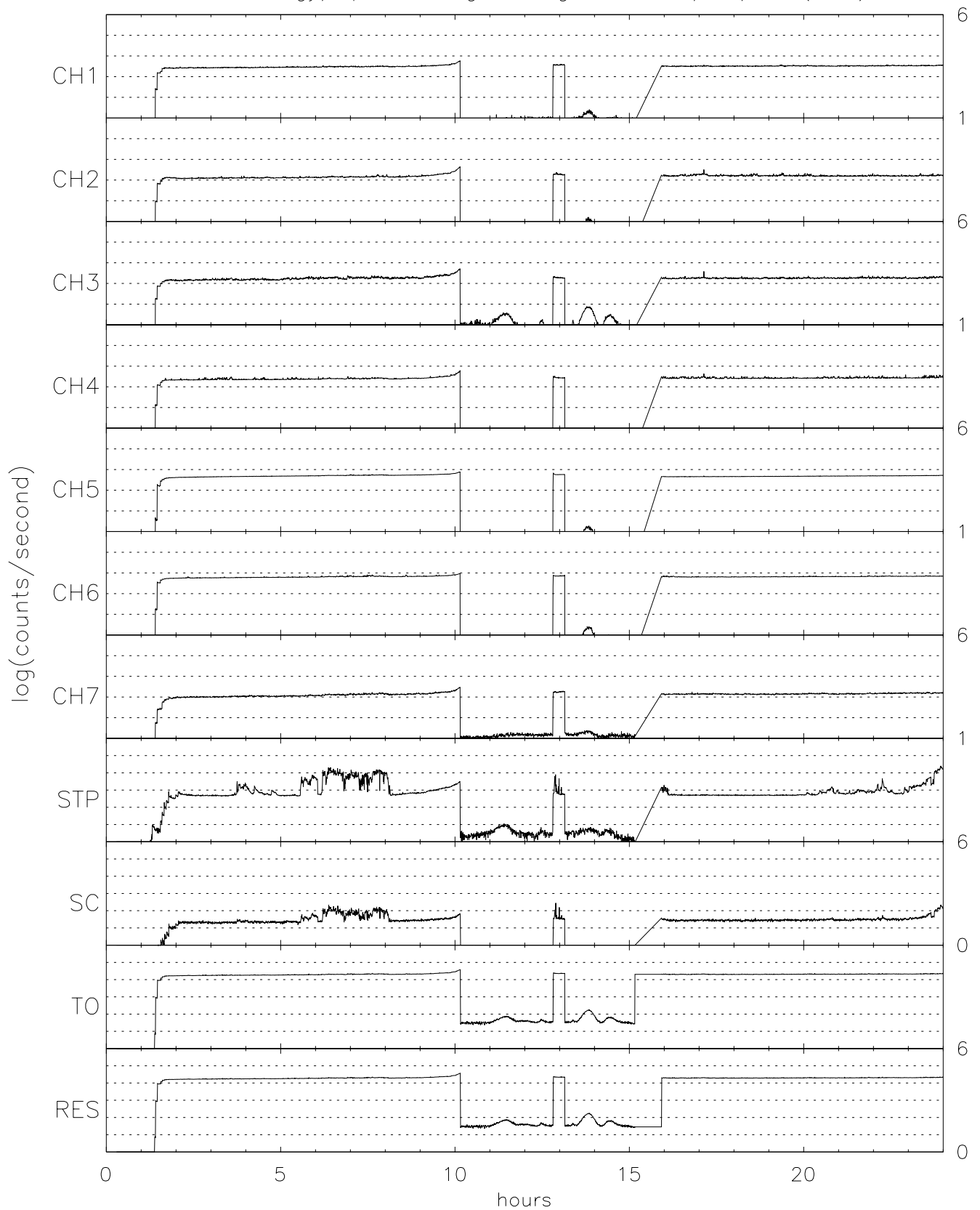
TIDE energy/spin averaged Singles for 10/24/96 (298)
