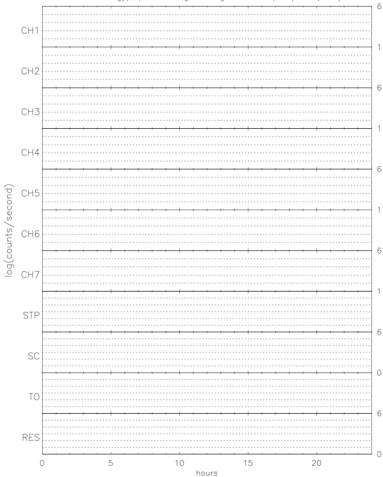
TIDE energy/spin averaged Singles for 10/19/96 (293)
