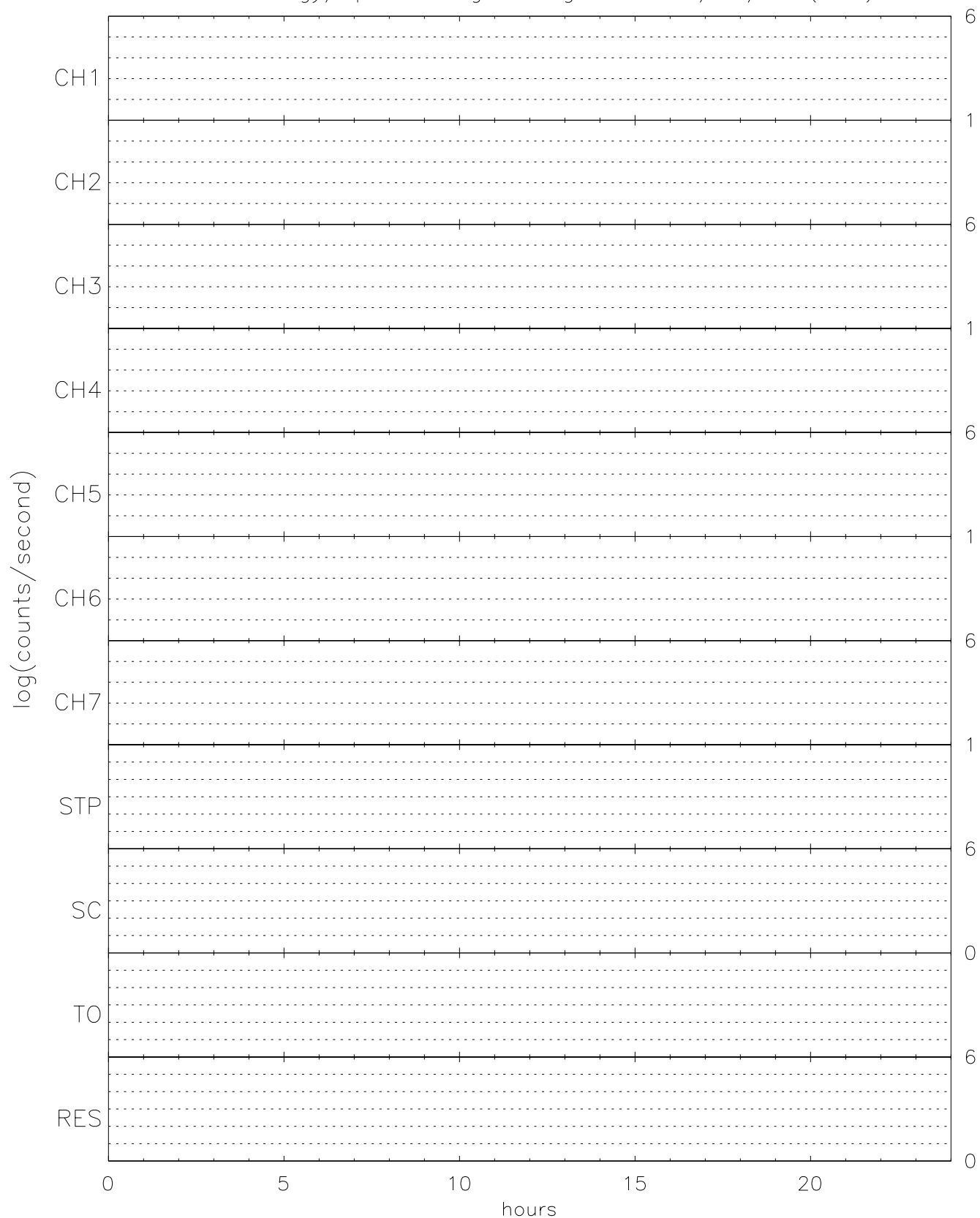
TIDE energy/spin averaged Singles for 10/17/96 (291)
