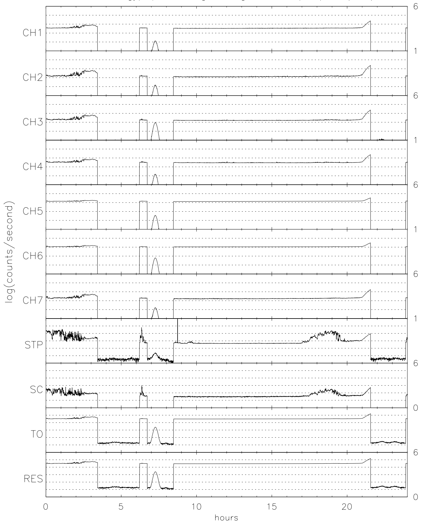
TIDE energy/spin averaged Singles for 10/14/96 (288)
