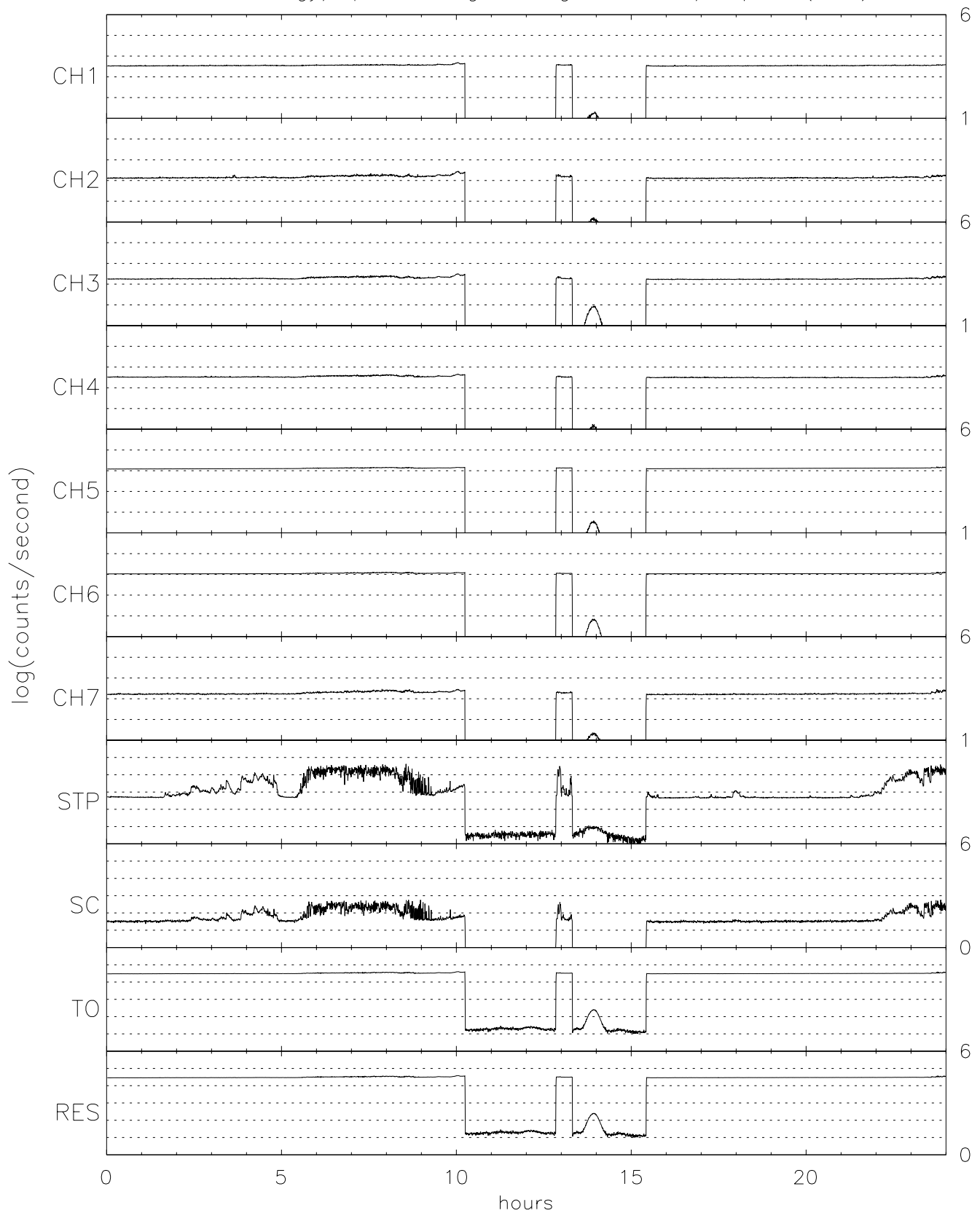
TIDE energy/spin averaged Singles for 10/13/96 (287)
