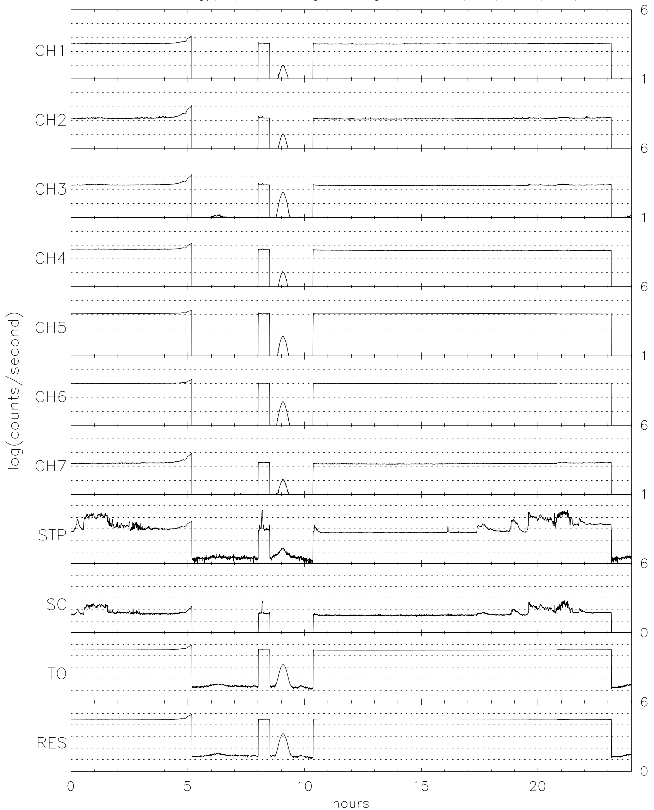
TIDE energy/spin averaged Singles for 10/11/96 (285)
