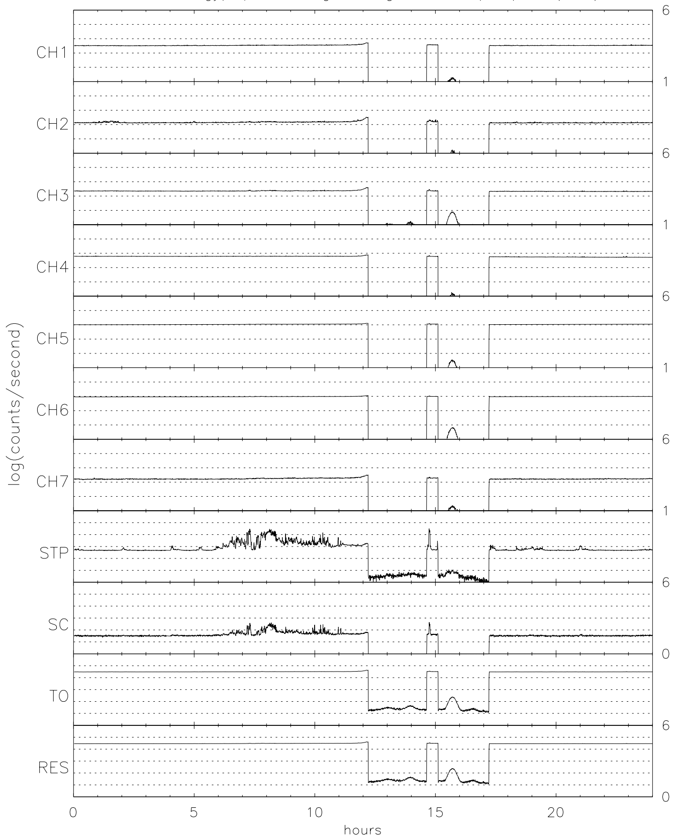
TIDE energy/spin averaged Singles for 10/10/96 (284)
