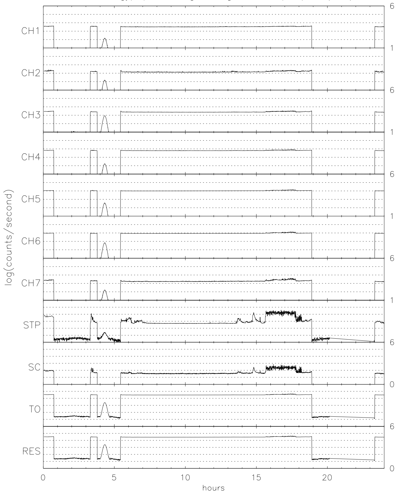
TIDE energy/spin averaged Singles for 10/09/96 (283)
