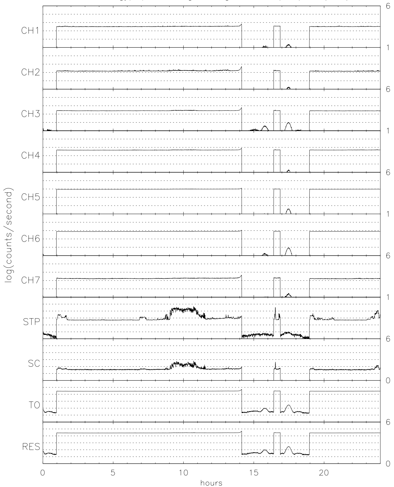
TIDE energy/spin averaged Singles for 10/07/96 (281)
