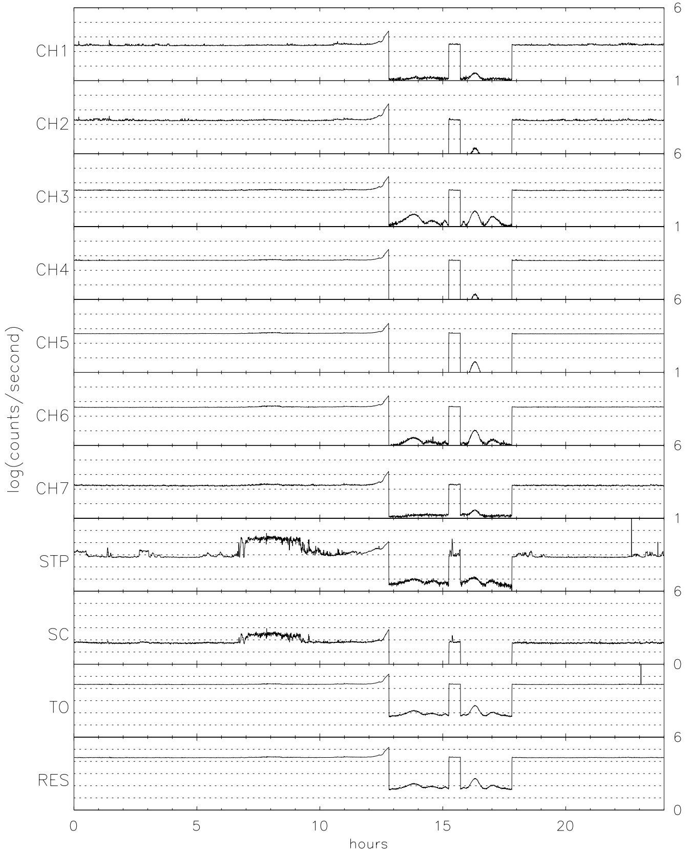
TIDE energy/spin averaged Singles for 09/29/96 (273)
