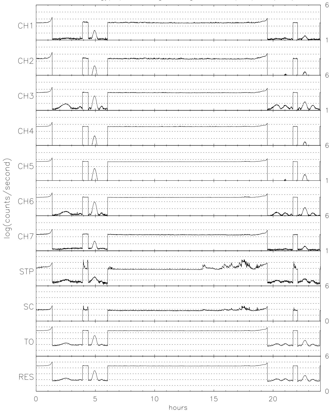
TIDE energy/spin averaged Singles for 09/28/96 (272)
