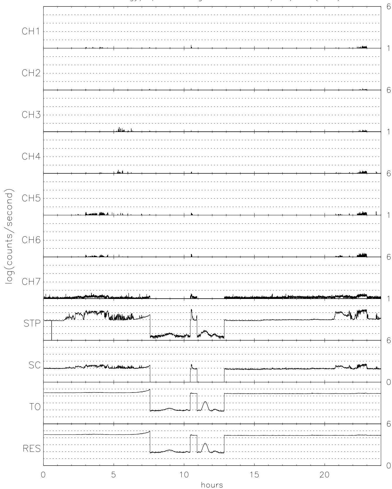
TIDE energy/spin averaged H+ for 09/27/96 (271)
