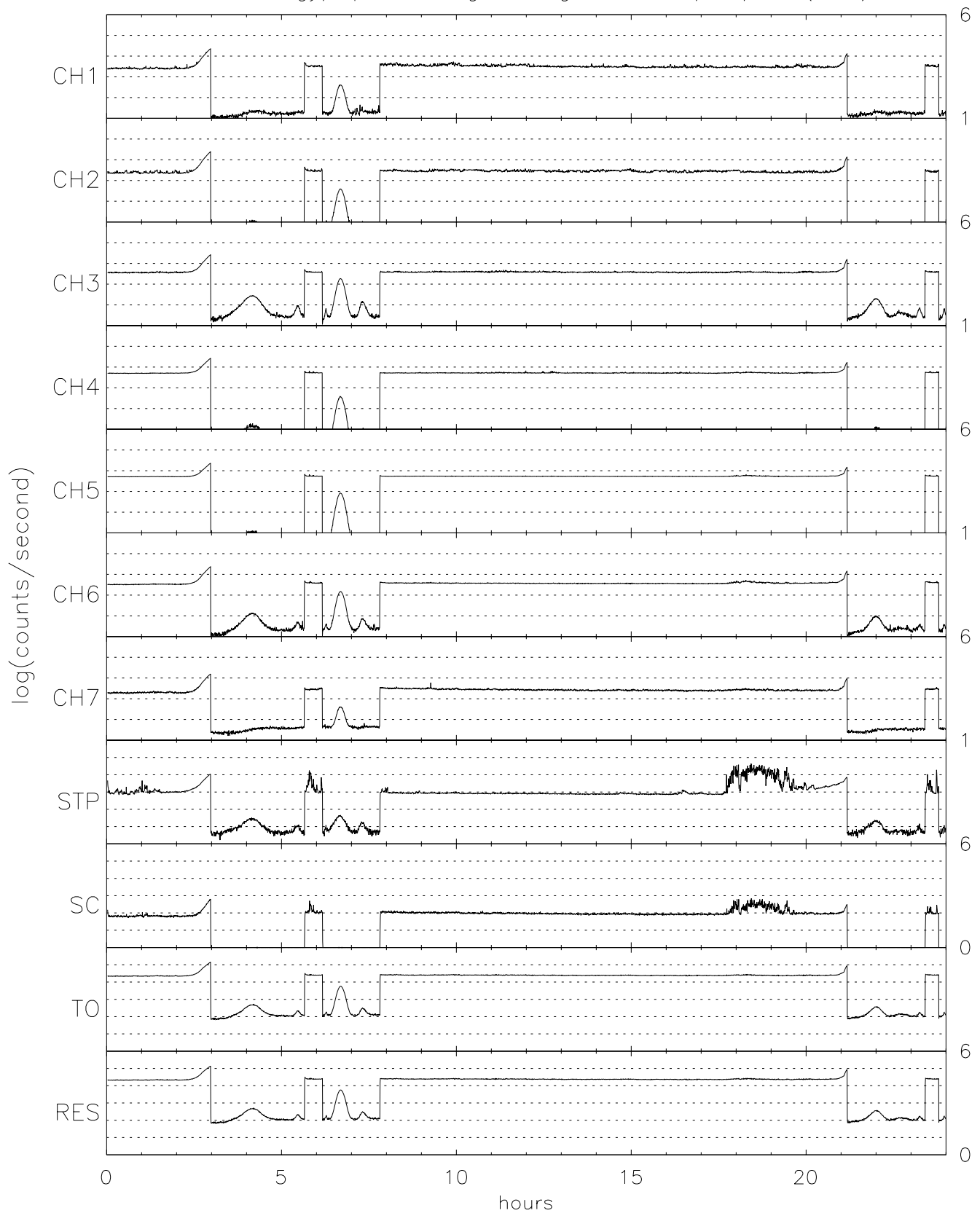
TIDE energy/spin averaged Singles for 09/25/96 (269)
