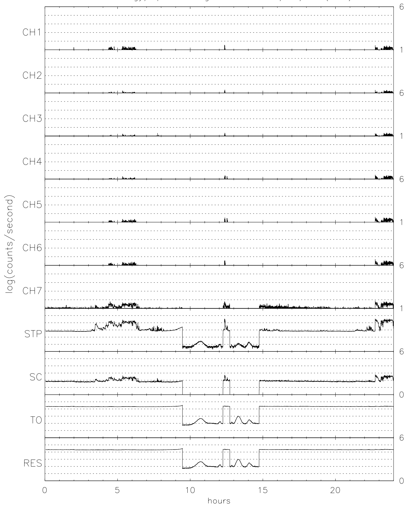
TIDE energy/spin averaged H+ for 09/24/96 (268)
