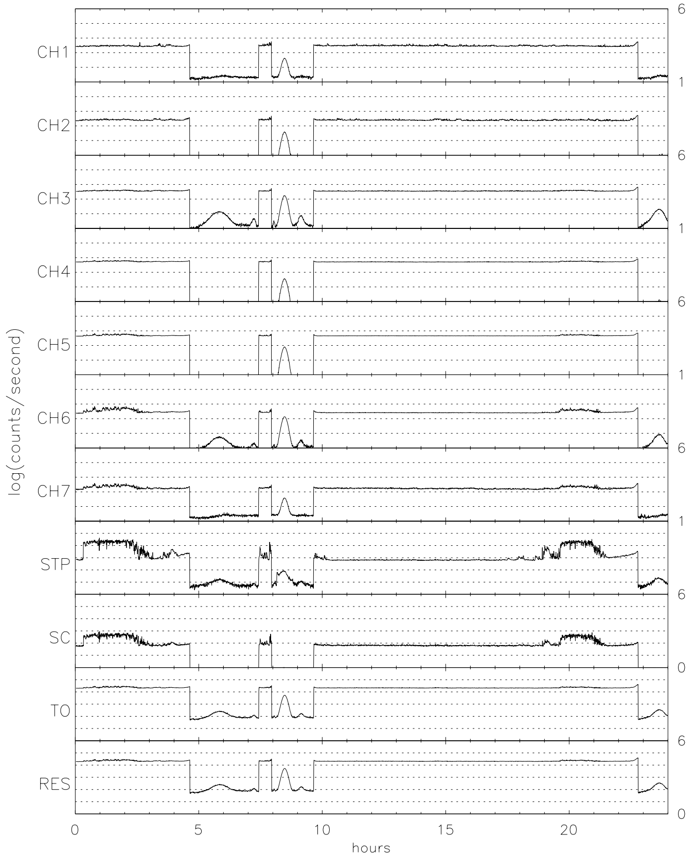
TIDE energy/spin averaged Singles for 09/22/96 (266)
