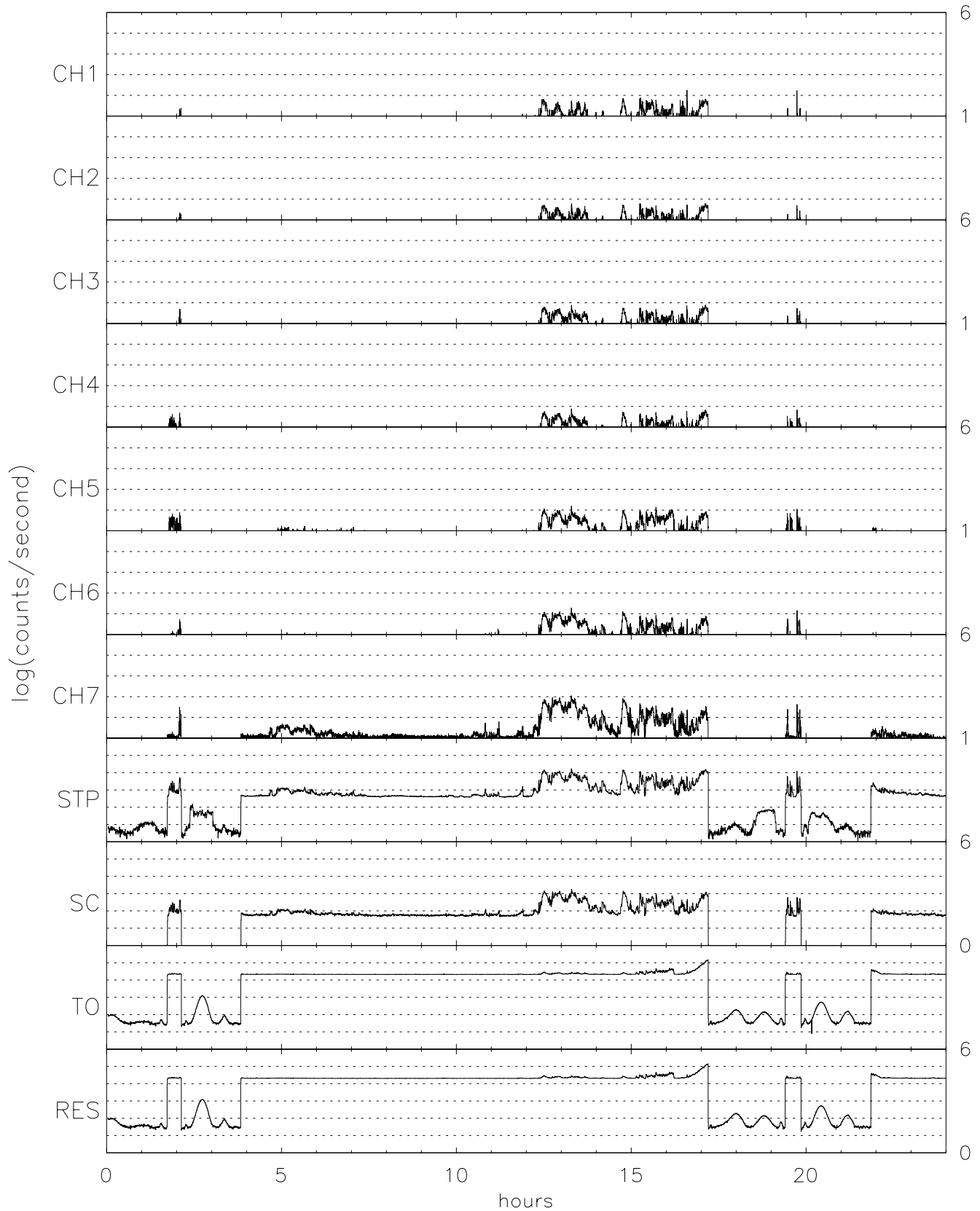
TIDE energy/spin averaged H+ for 09/12/96 (256)
