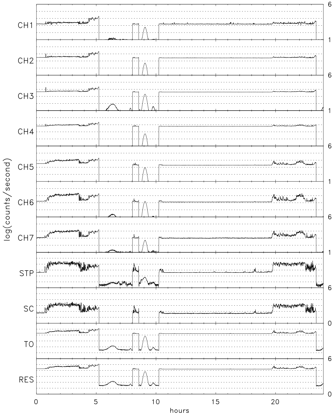
TIDE energy/spin averaged Singles for 09/11/96 (255)
