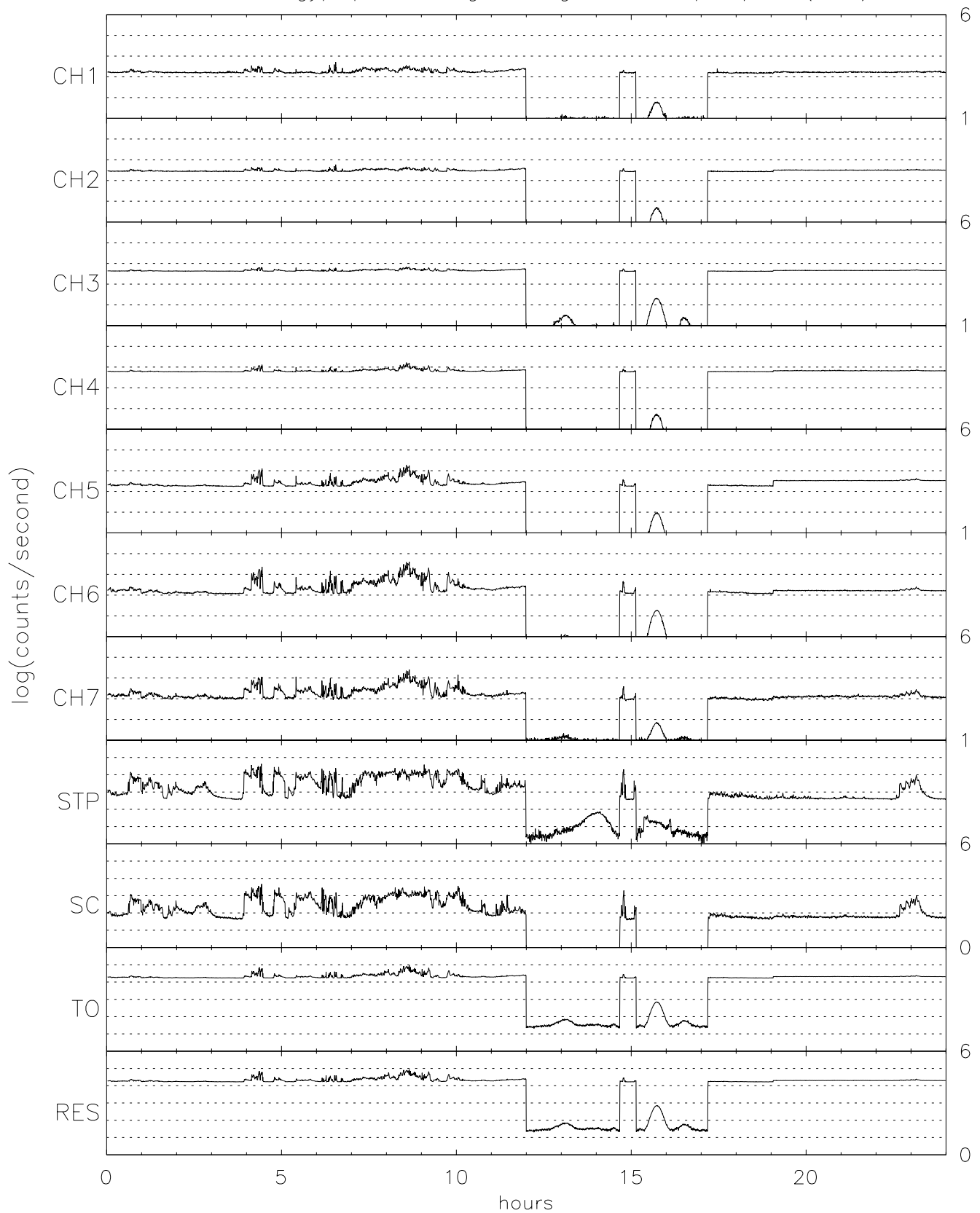
TIDE energy/spin averaged Singles for 09/10/96 (254)
