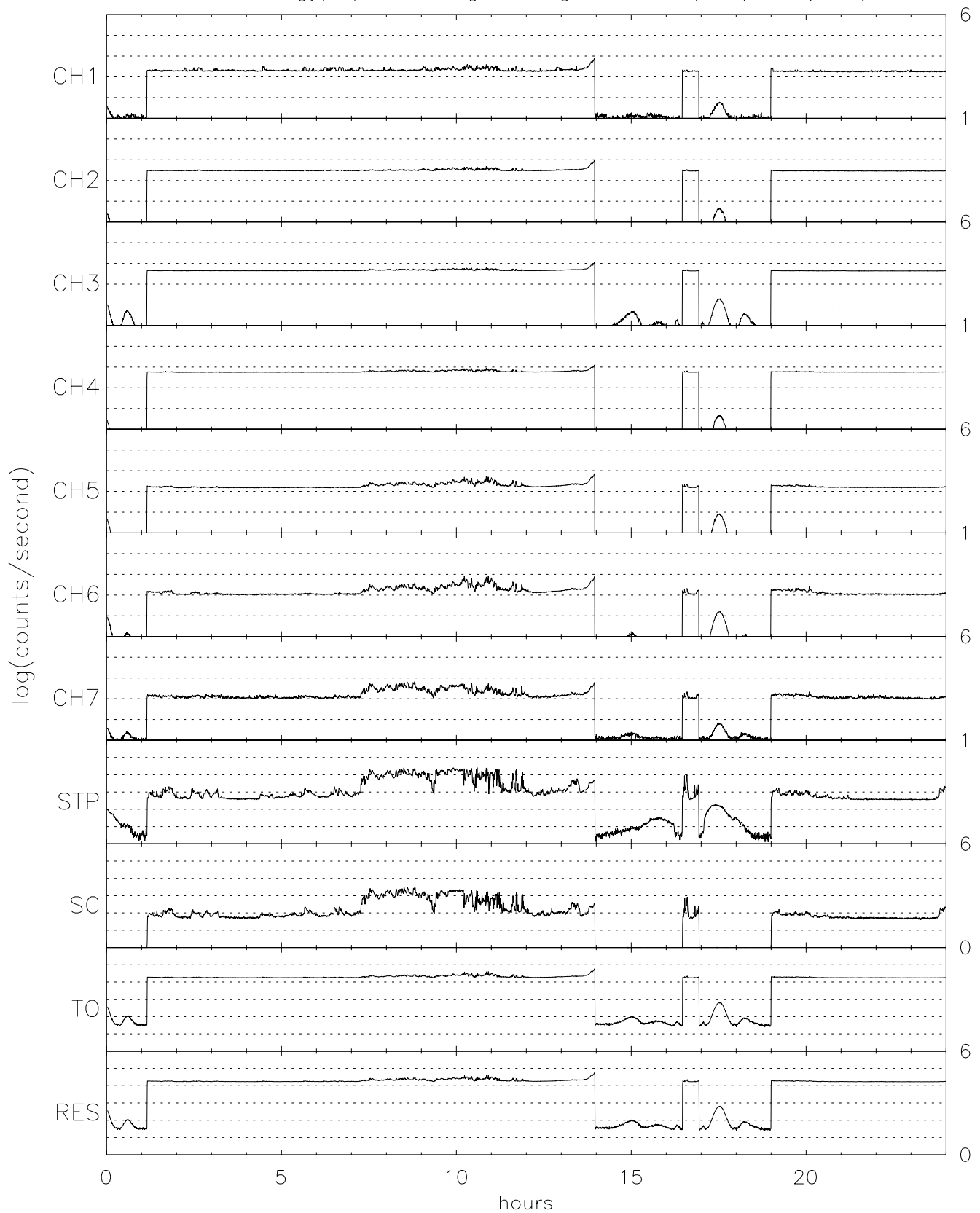
TIDE energy/spin averaged Singles for 09/07/96 (251)
