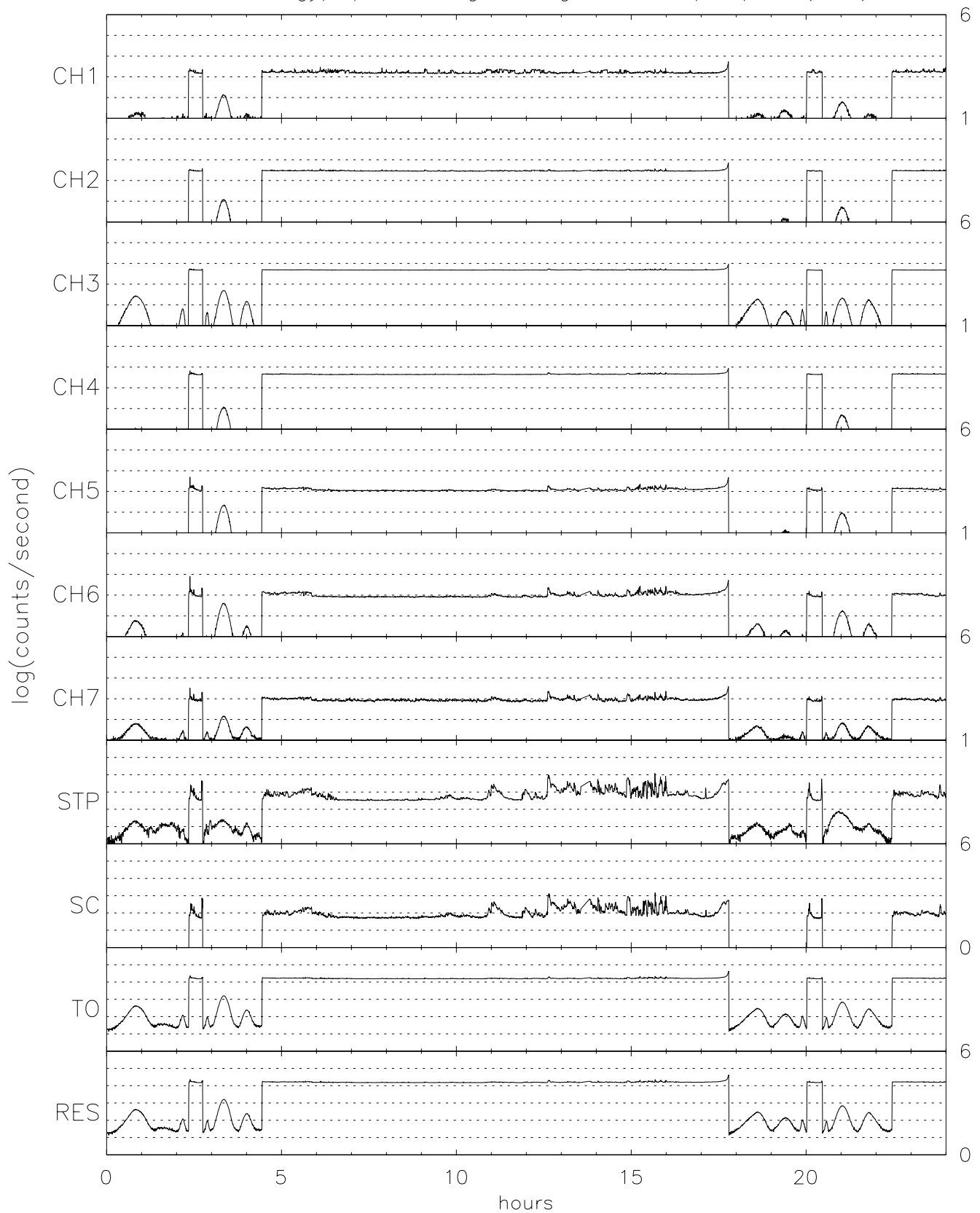
TIDE energy/spin averaged Singles for 09/01/96 (245)
