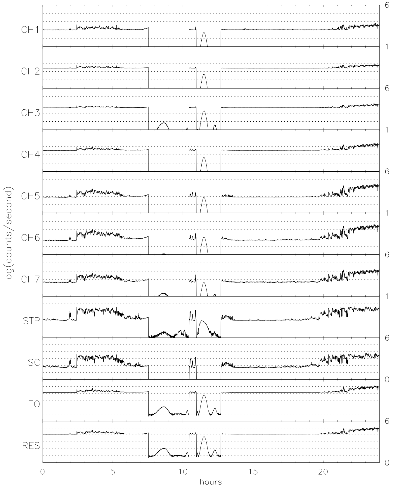
TIDE energy/spin averaged Singles for 08/28/96 (241)
