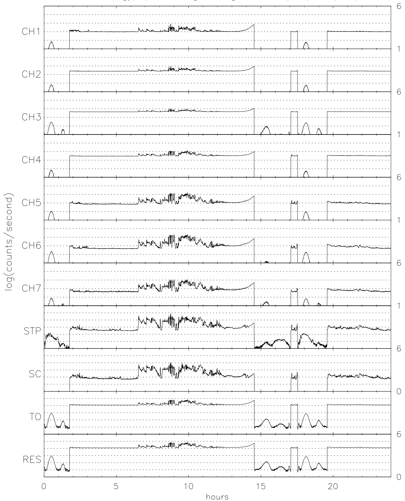
TIDE energy/spin averaged Singles for 08/27/96 (240)
