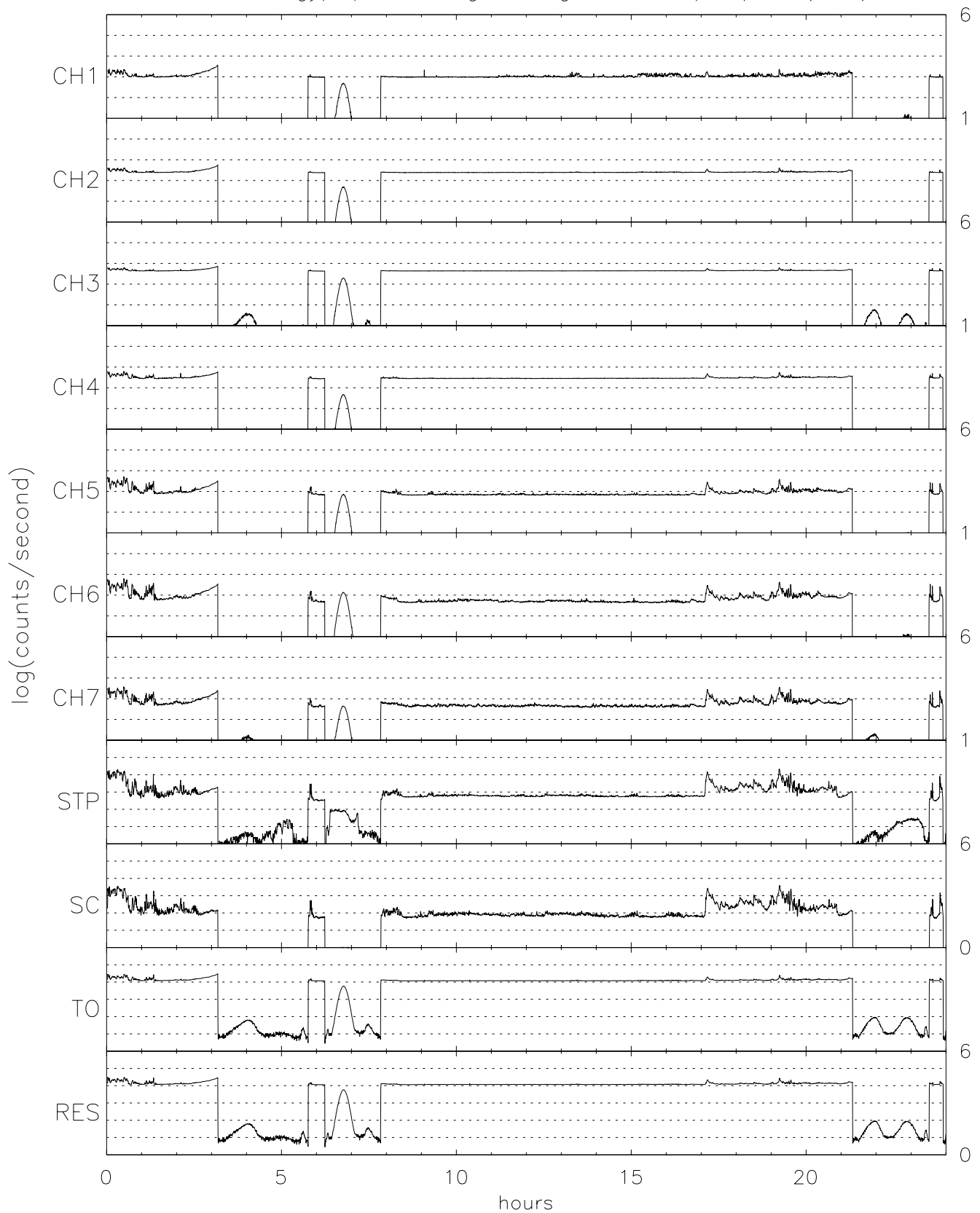
TIDE energy/spin averaged Singles for 08/26/96 (239)
