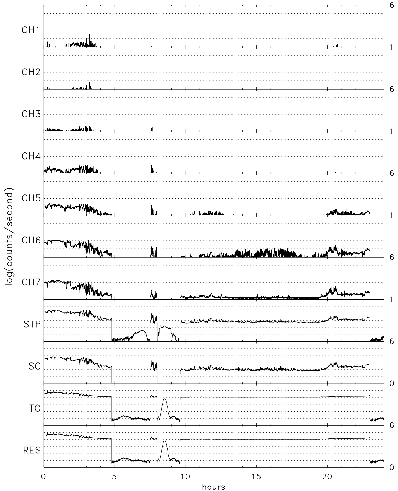
TIDE energy/spin averaged H+ for 08/23/96 (236)
