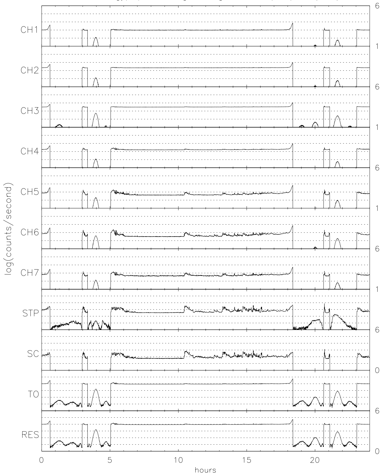
TIDE energy/spin averaged Singles for 08/21/96 (234)
