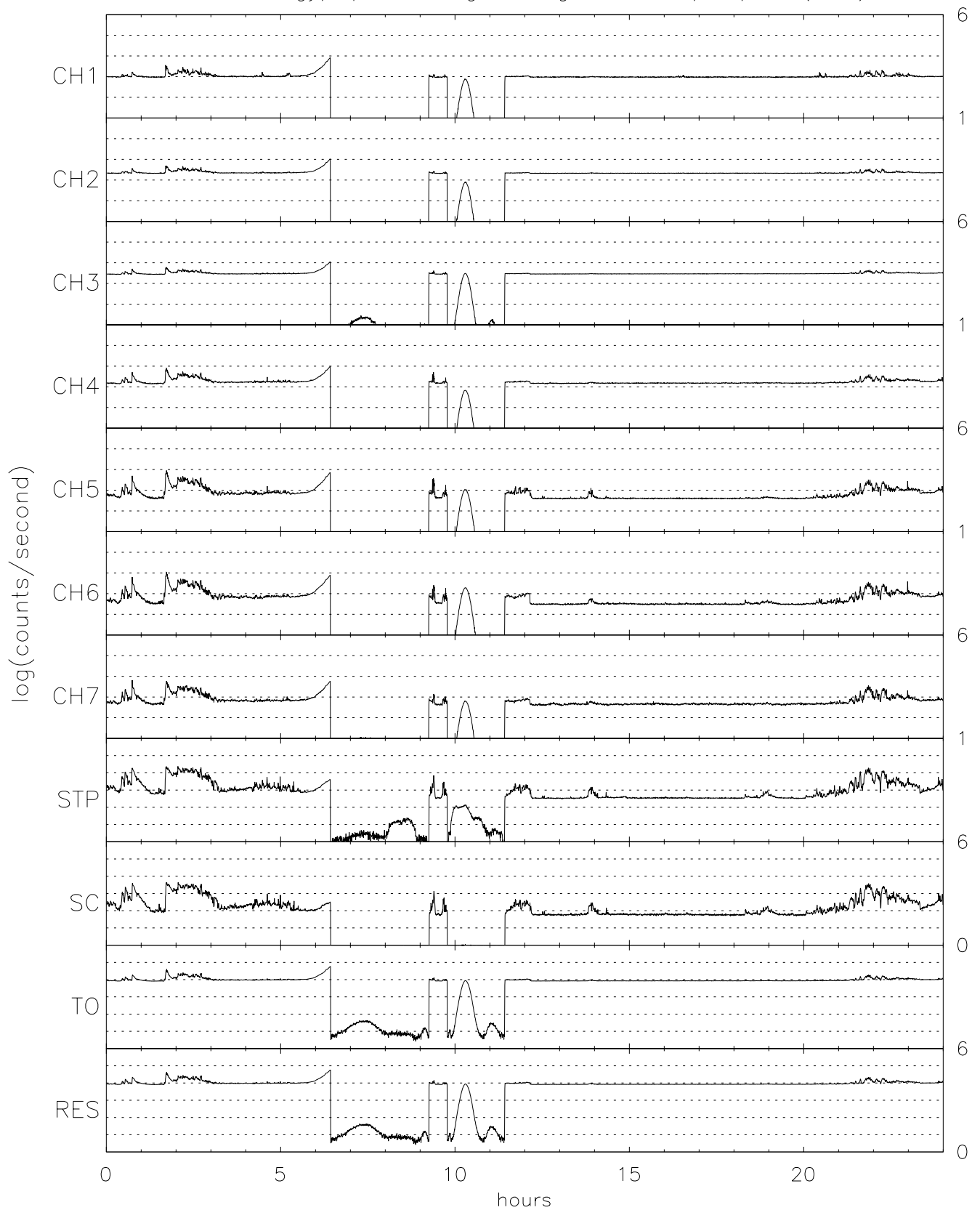
TIDE energy/spin averaged Singles for 08/20/96 (233)
