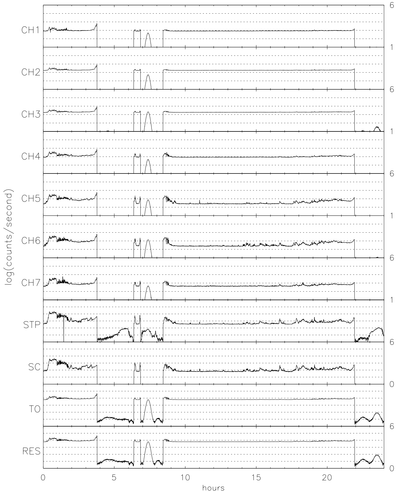
TIDE energy/spin averaged Singles for 08/15/96 (228)
