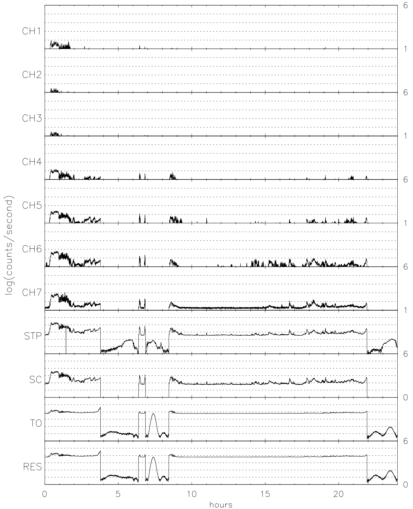
TIDE energy/spin averaged H+ for 08/15/96 (228)
