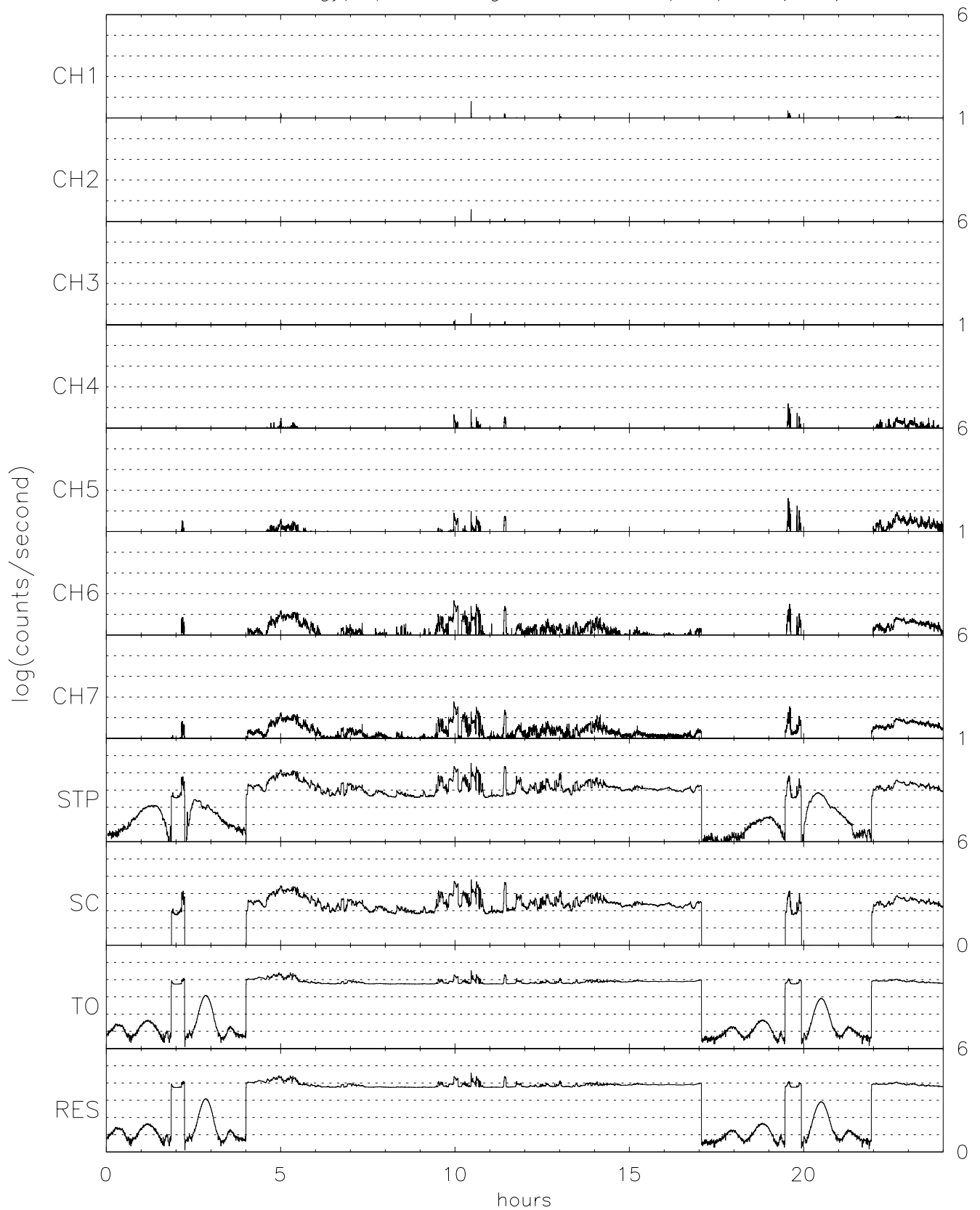
TIDE energy/spin averaged H+ for 08/13/96 (226)
