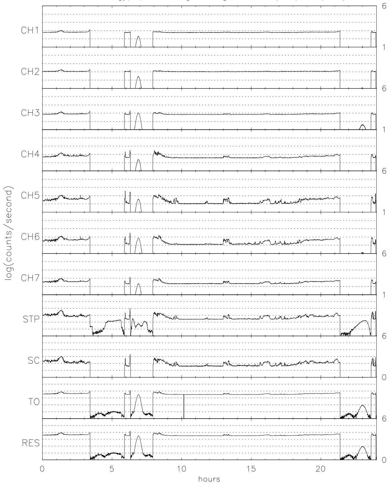
TIDE energy/spin averaged Singles for 07/27/96 (209)
