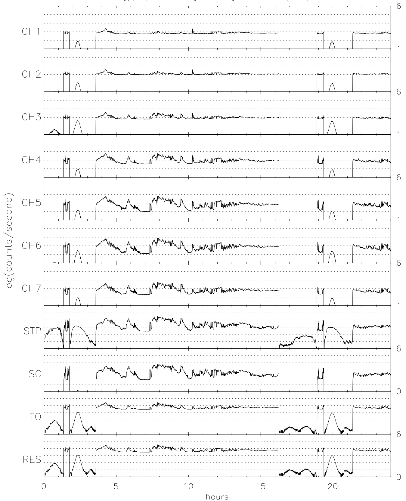
TIDE energy/spin averaged Singles for 07/25/96 (207)
