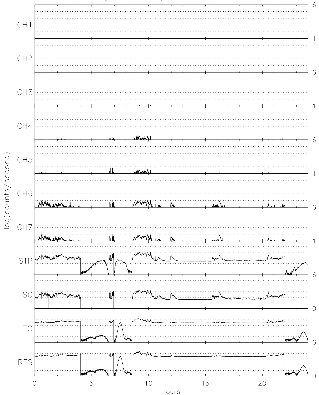
TIDE energy/spin averaged H+ for 07/16/96 (198)
