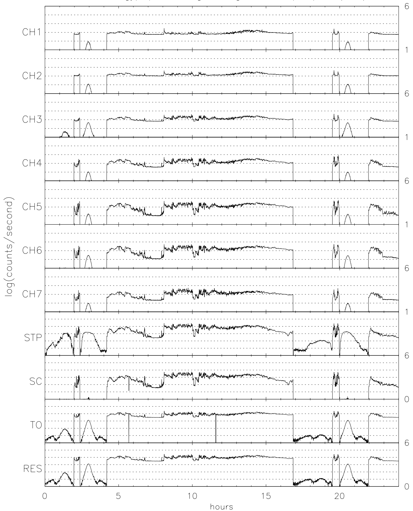
TIDE energy/spin averaged Singles for 07/14/96 (196)
