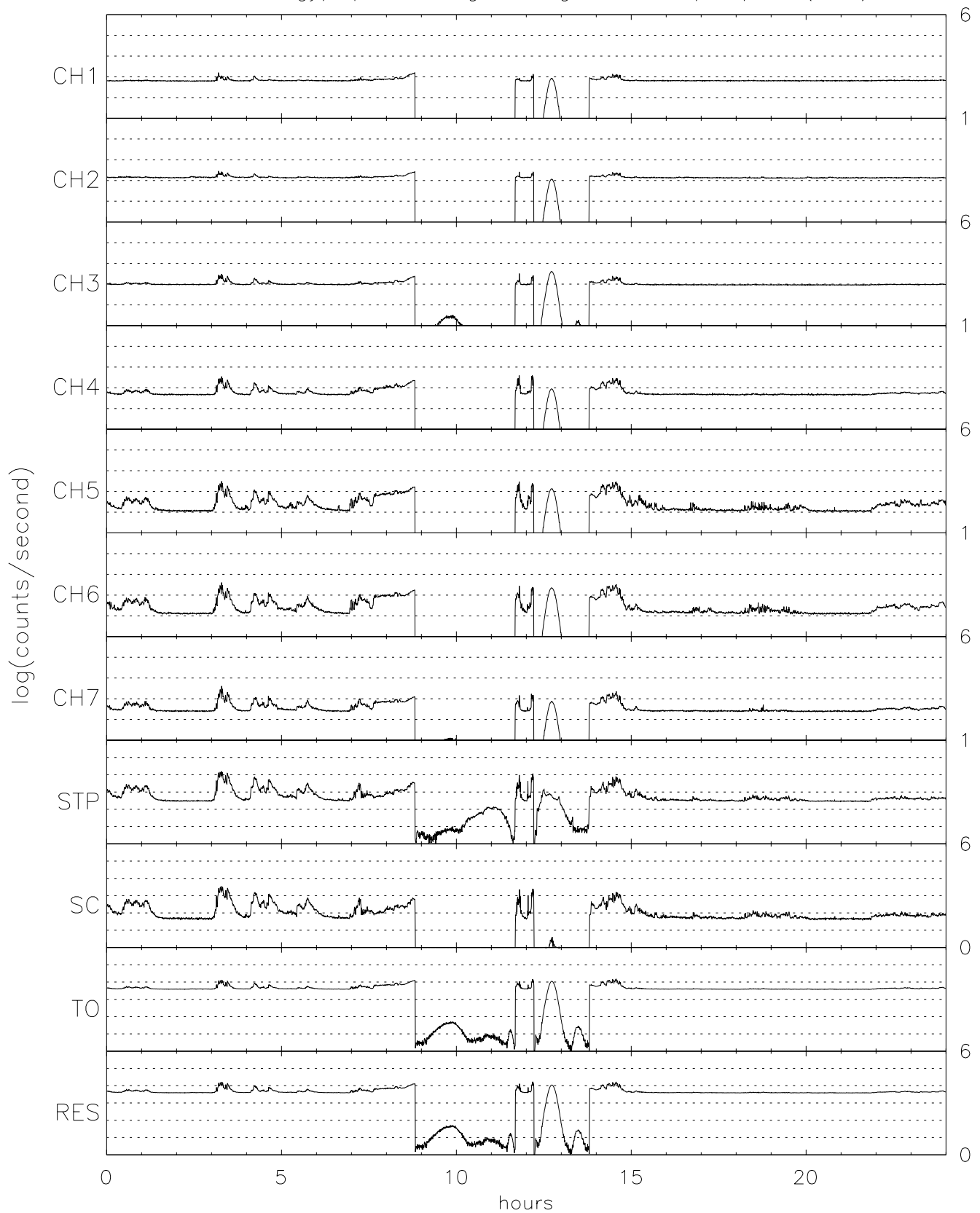
TIDE energy/spin averaged Singles for 07/07/96 (189)
