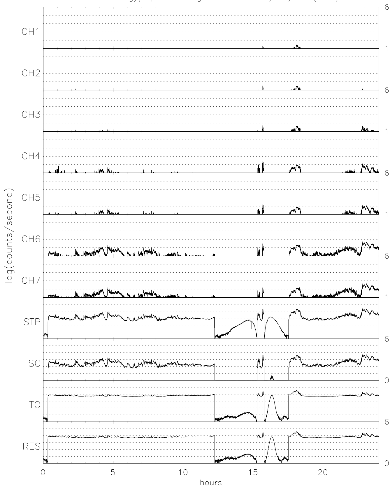
TIDE energy/spin averaged H+ for 07/01/96 (183)
