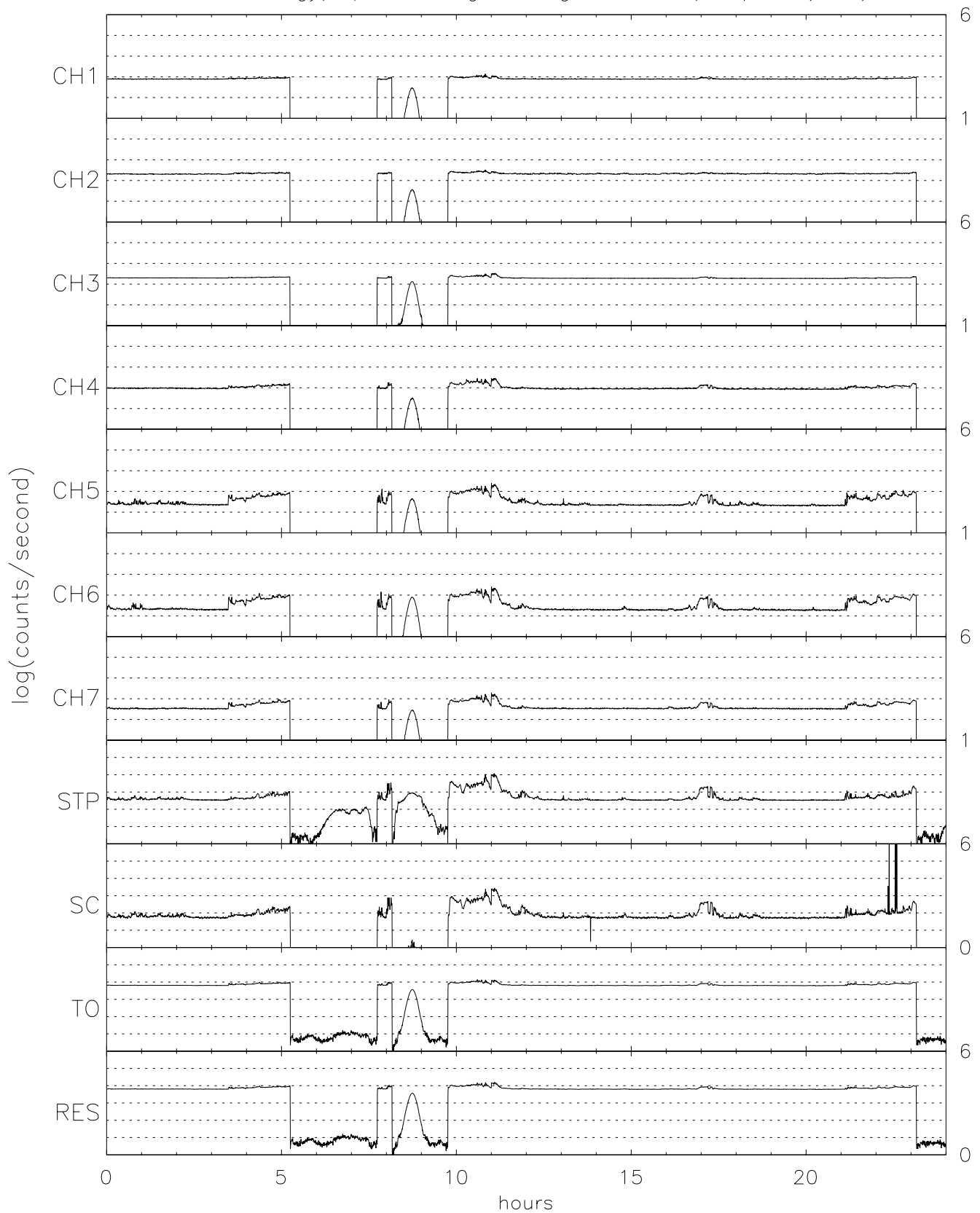
TIDE energy/spin averaged Singles for 06/24/96 (176)
