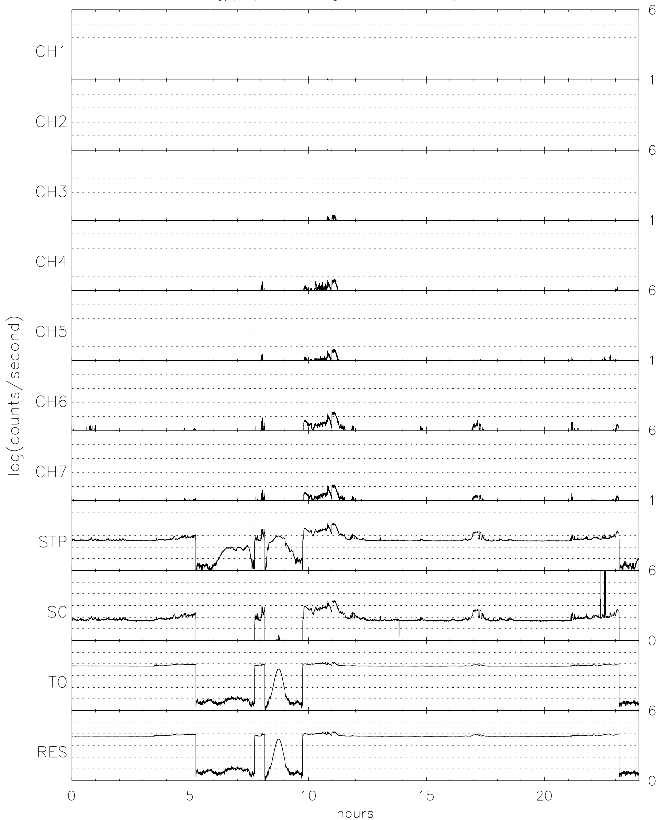
TIDE energy/spin averaged H+ for 06/24/96 (176)
