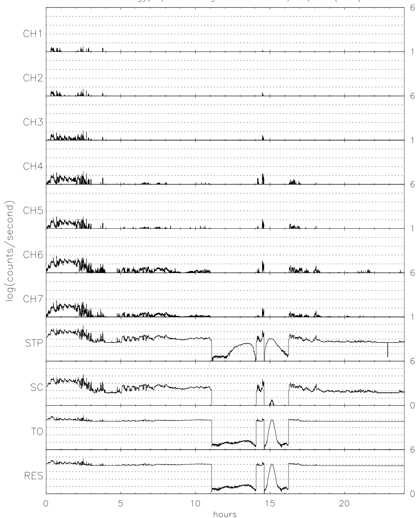
TIDE energy/spin averaged H+ for 06/23/96 (175)
