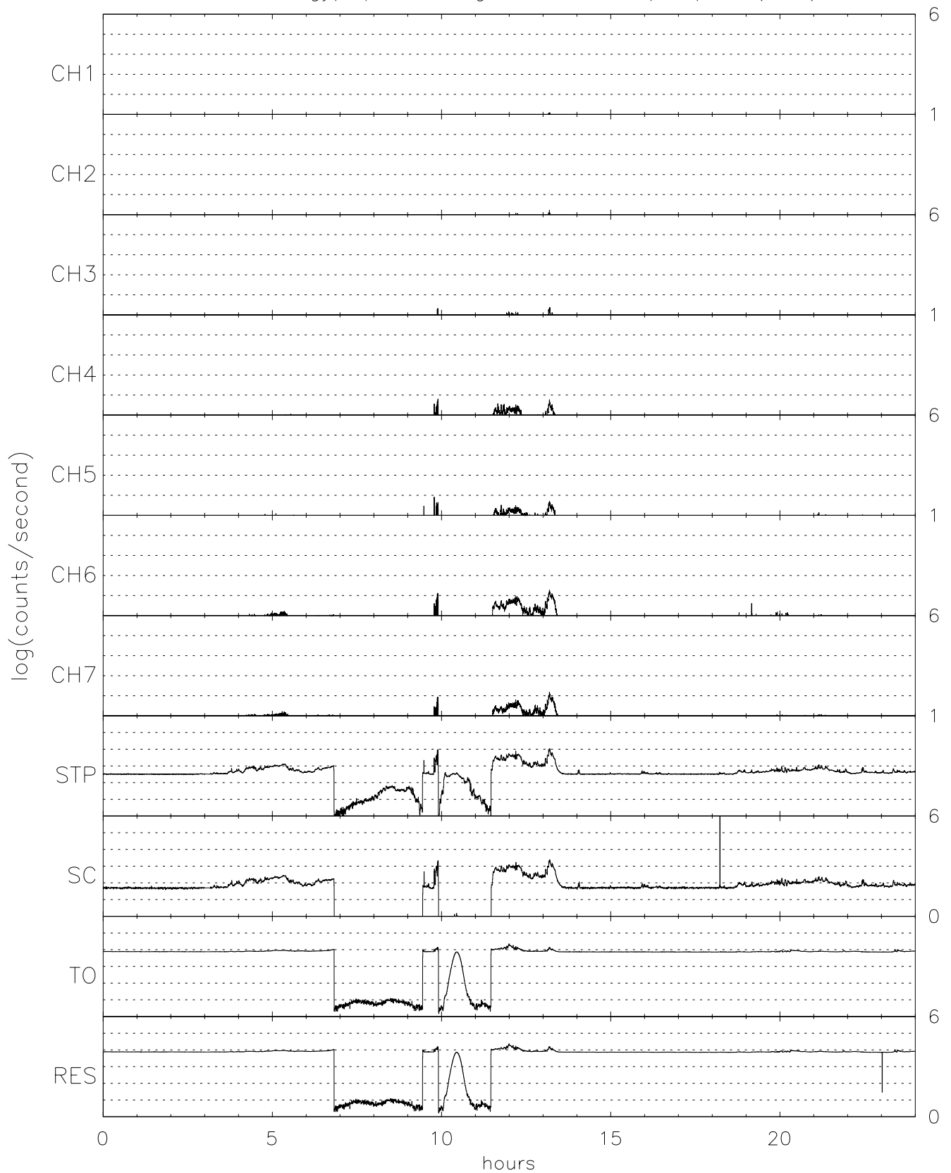
TIDE energy/spin averaged H+ for 06/21/96 (173)
